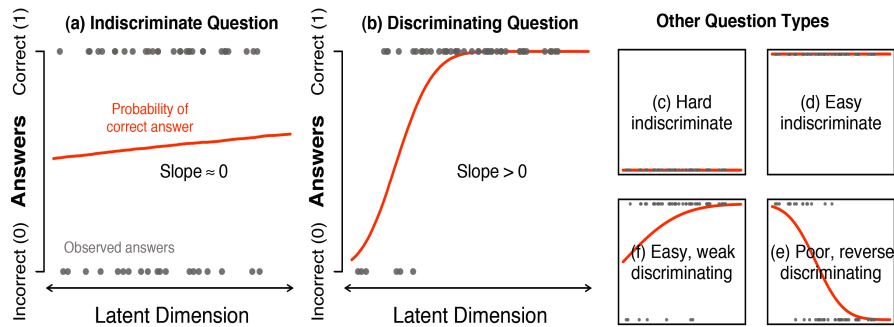
Figure 2: Estimating latent “intelligence” dimension from standardized test. Each panel represents a hypothetical test question that induces different responses. The x -axis represents the latent dimension of intelligence. The y -axis represents the probability of a correct answer, ranging from 0 to 1. The grey dots are the observed answers by fifty test takers, coded as 1 if correct and 0 if incorrect. The red curve plots the relationship between intelligence and test answers. The left panel (a) shows an indiscriminate test question, with a slope of the relationship between intelligence and answers close to 0. The middle panel (b) represents a question that discriminates quite well between more and less intelligent test takers. The slope is sharply positive, and the only test takers incorrectly answering the question are at the low end of the latent dimension. The four panels on the right display other types of test questions. From top left, clockwise: (c) a hard, indiscriminate question no one answers correctly; (d) an easy, indiscriminate question everyone answers correctly; (e) a poor question that intelligent test takers overthink and therefore are more likely to answer incorrectly; (f) an easy, weakly discriminating question that less intelligent student have a low probability of answering incorrectly.
